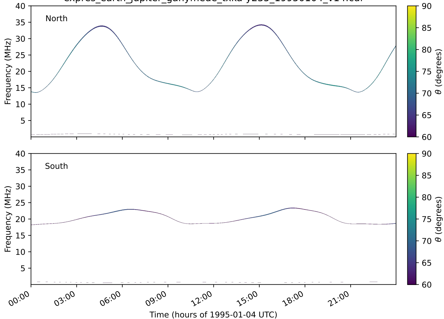
expres_earth_jupiter_ganymede_txka-y235_19950104_v14.cdf
