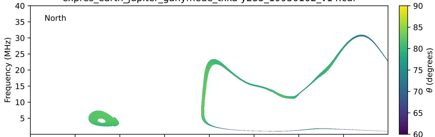
expres_earth_jupiter_ganymede_txka-y235_19950102_v14.cdf
