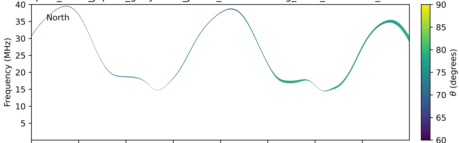
expres_earth_jupiter_ganymede_jrm33_lossc-wid1deg_3kev_19950112_v11.cdf
