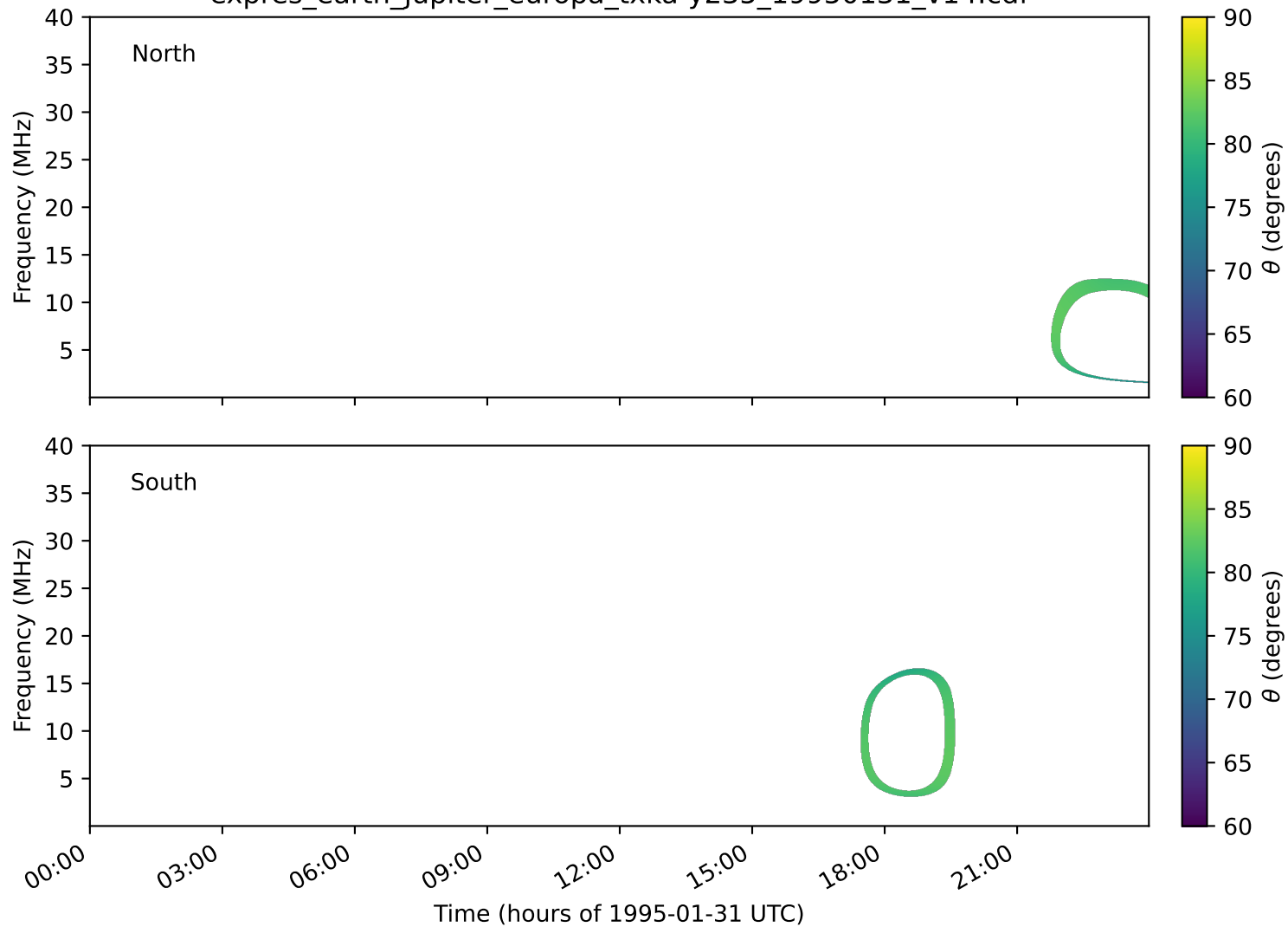
expres_earth_jupiter_europa_txka-y235_19950131_v14.cdf
