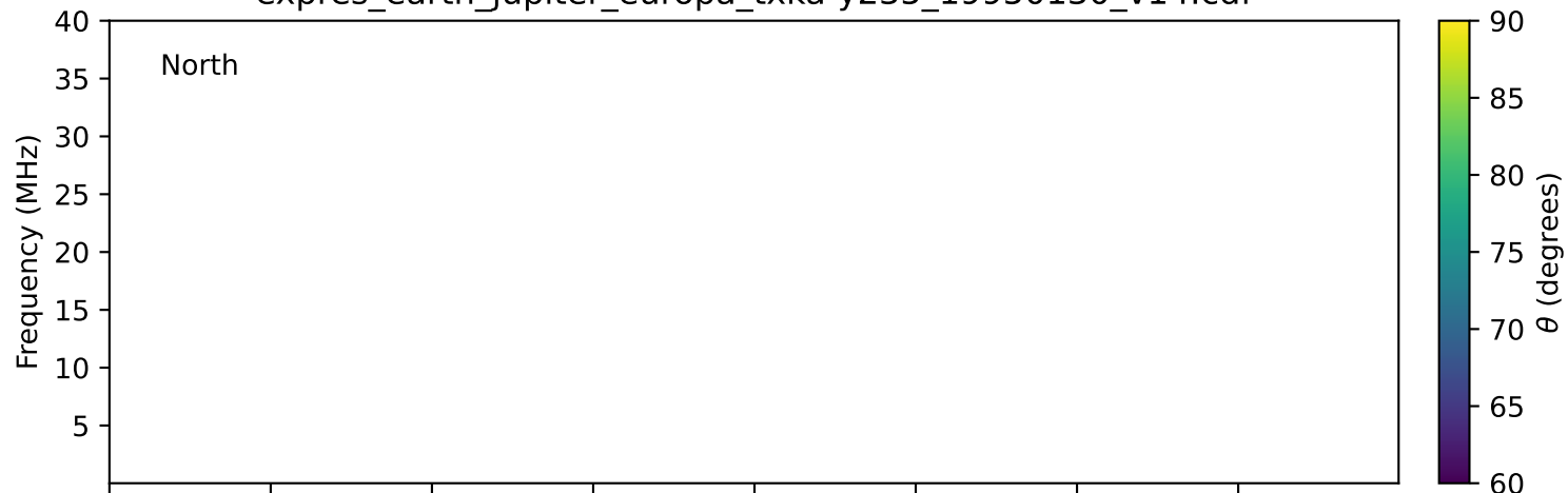
expres_earth_jupiter_europa_txka-y235_19950130_v14.cdf
