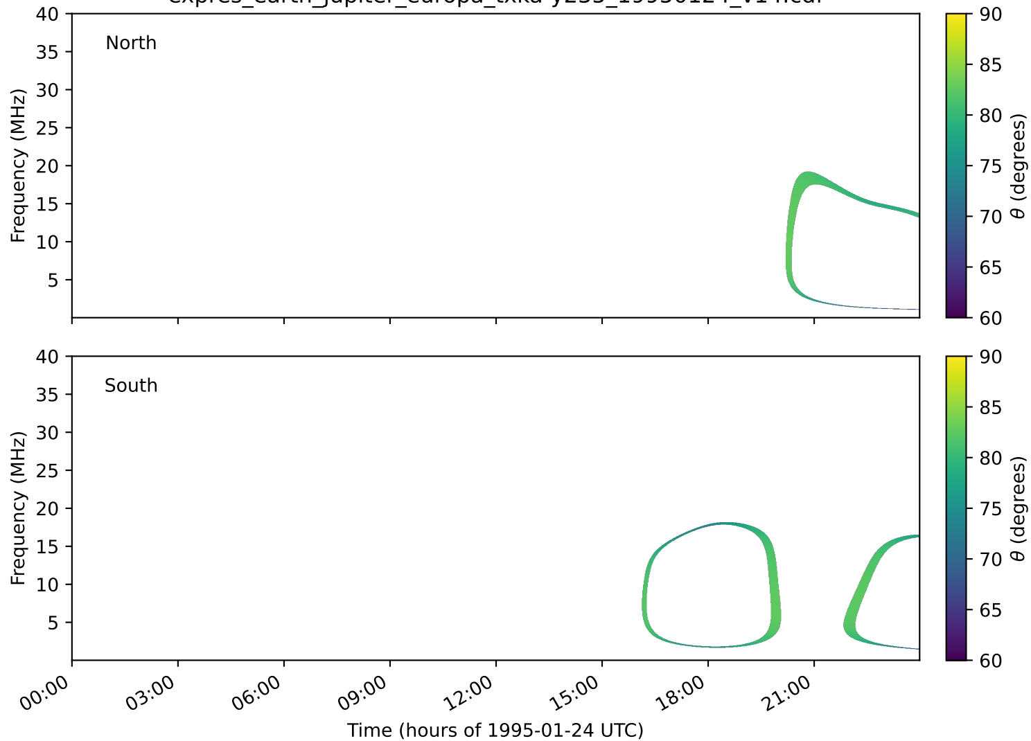
expres_earth_jupiter_europa_txka-y235_19950124_v14.cdf
