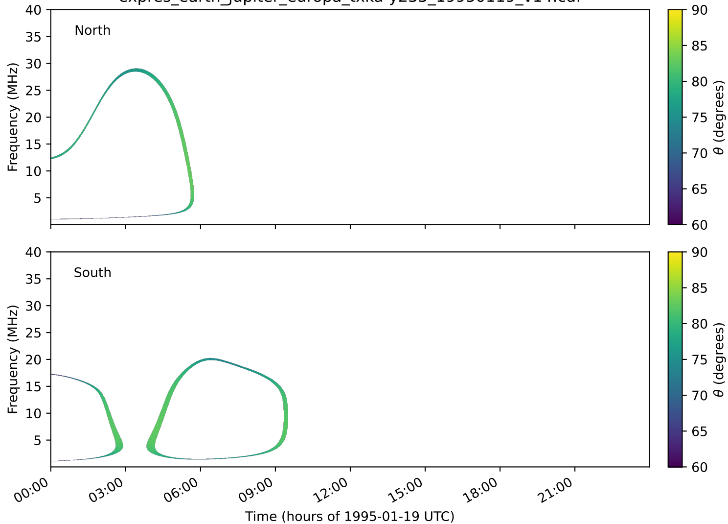
expres_earth_jupiter_europa_txka-y235_19950119_v14.cdf
