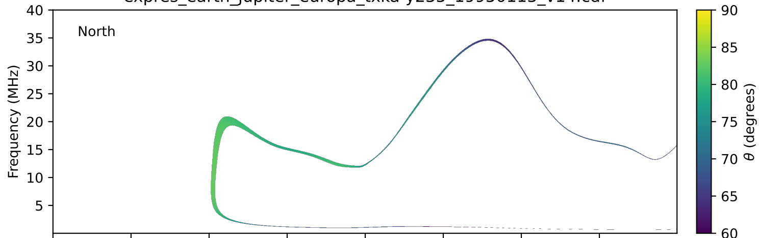
expres_earth_jupiter_europa_txka-y235_19950113_v14.cdf
