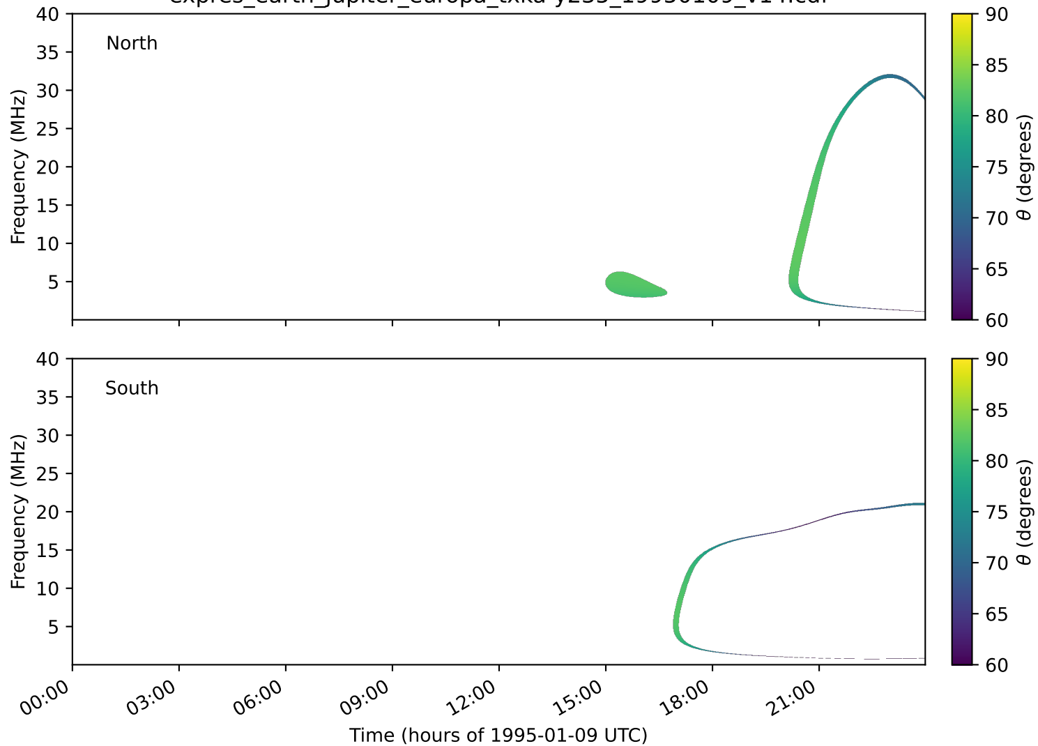
expres_earth_jupiter_europa_txka-y235_19950109_v14.cdf
