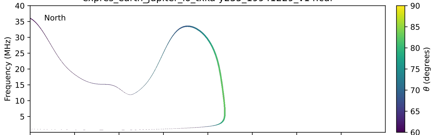
expres_earth_jupiter_io_txka-y235_19941229_v14.cdf
