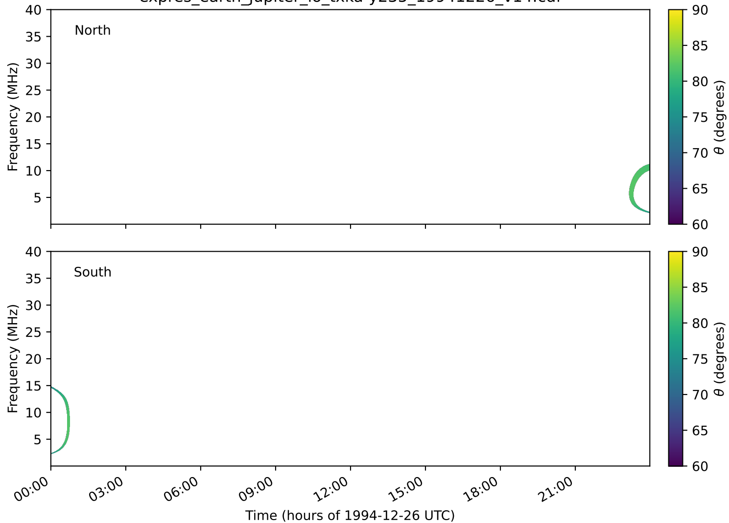
expres_earth_jupiter_io_txka-y235_19941226_v14.cdf
