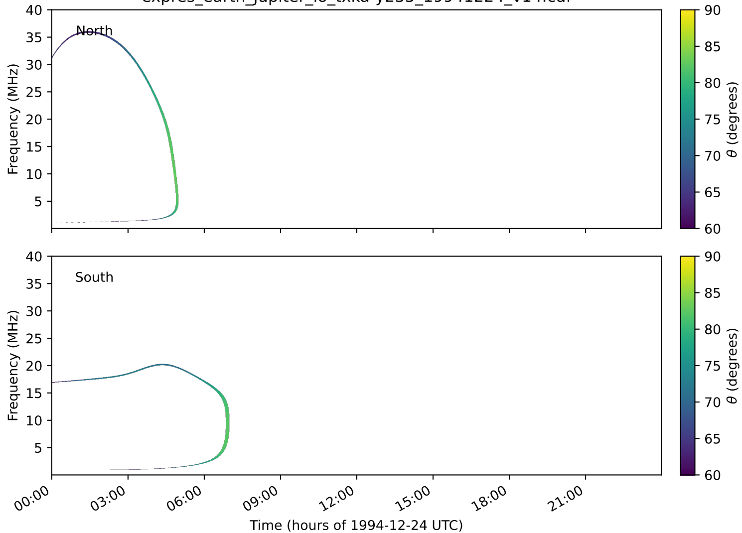
expres_earth_jupiter_io_txka-y235_19941224_v14.cdf
