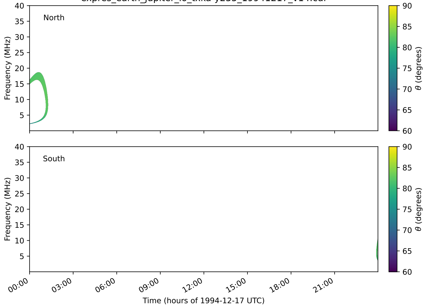
expres_earth_jupiter_io_txka-y235_19941217_v14.cdf
