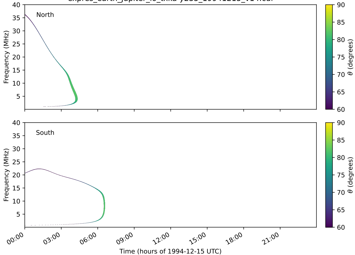
expres_earth_jupiter_io_txka-y235_19941215_v14.cdf
