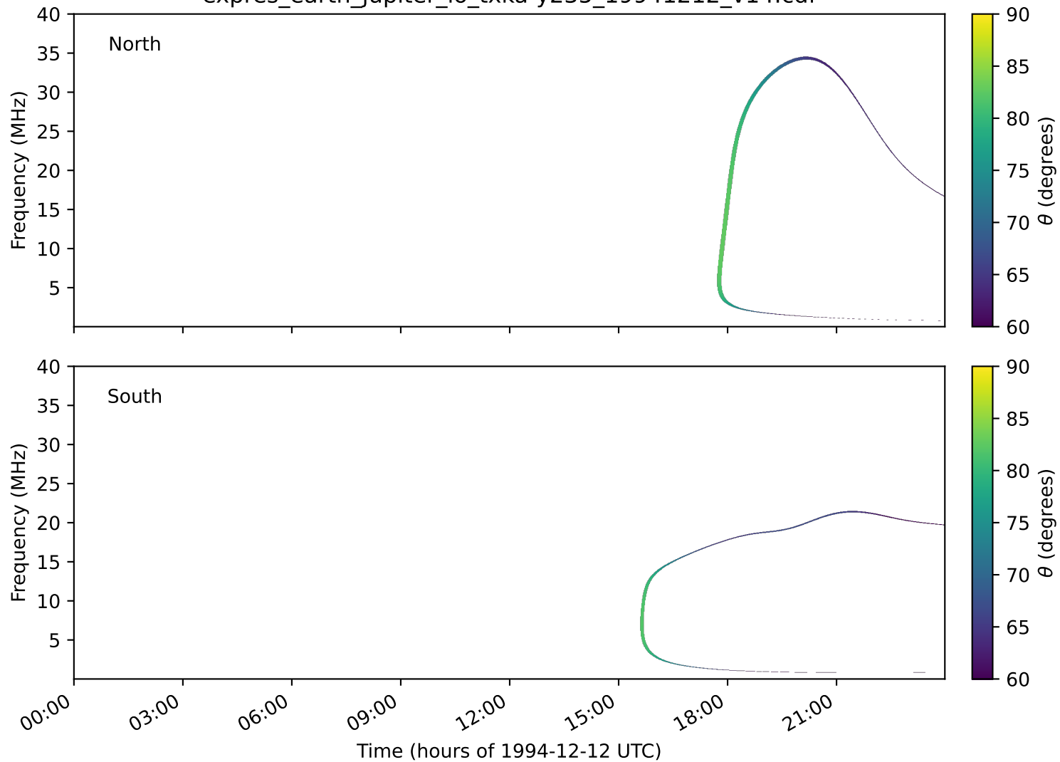
expres_earth_jupiter_io_txka-y235_19941212_v14.cdf
