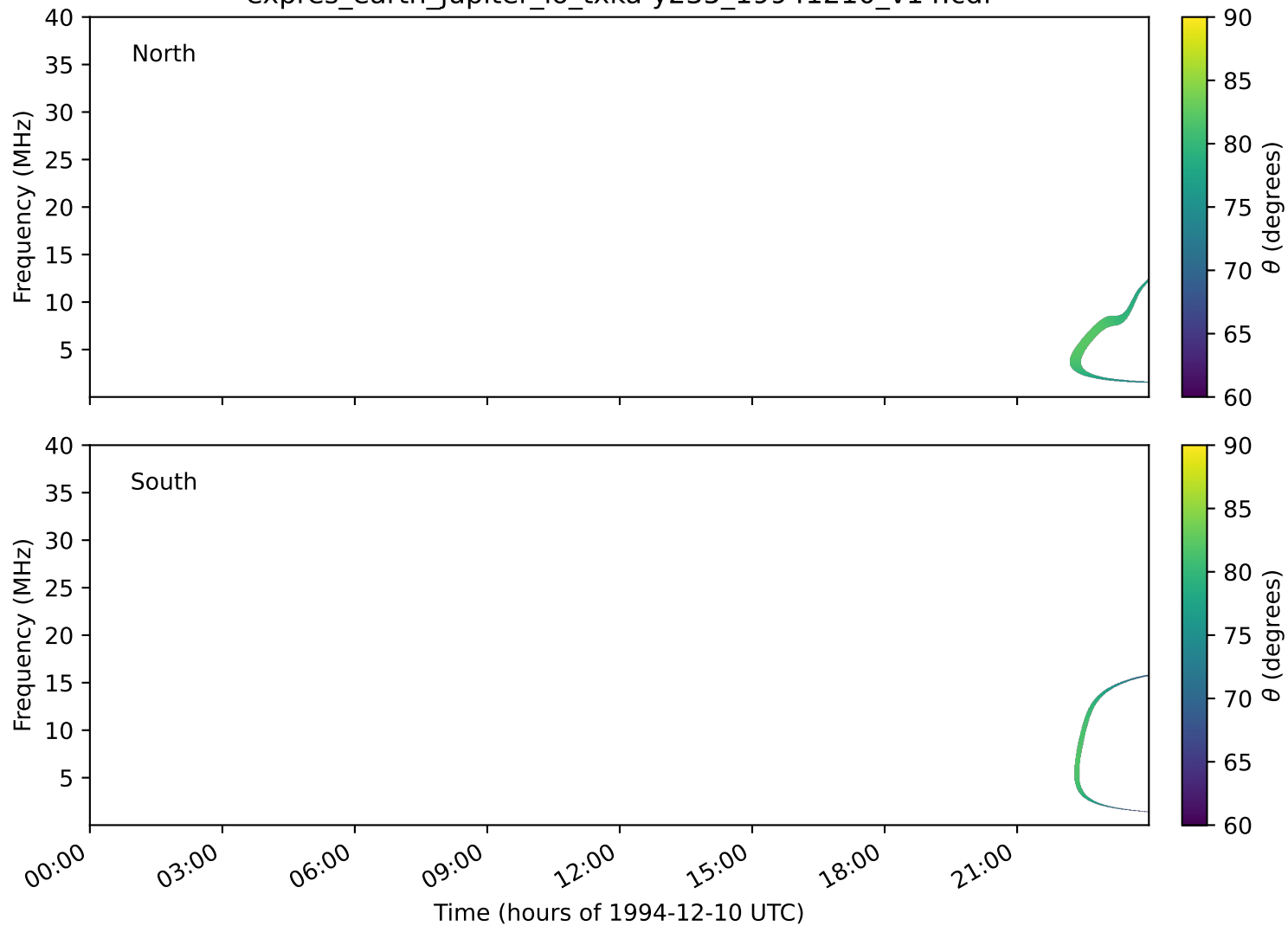
expres_earth_jupiter_io_txka-y235_19941210_v14.cdf
