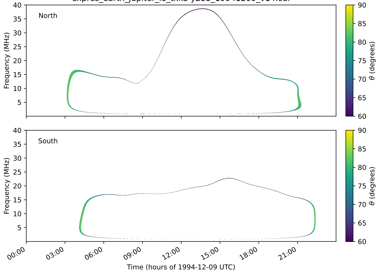
expres_earth_jupiter_io_txka-y235_19941209_v14.cdf
