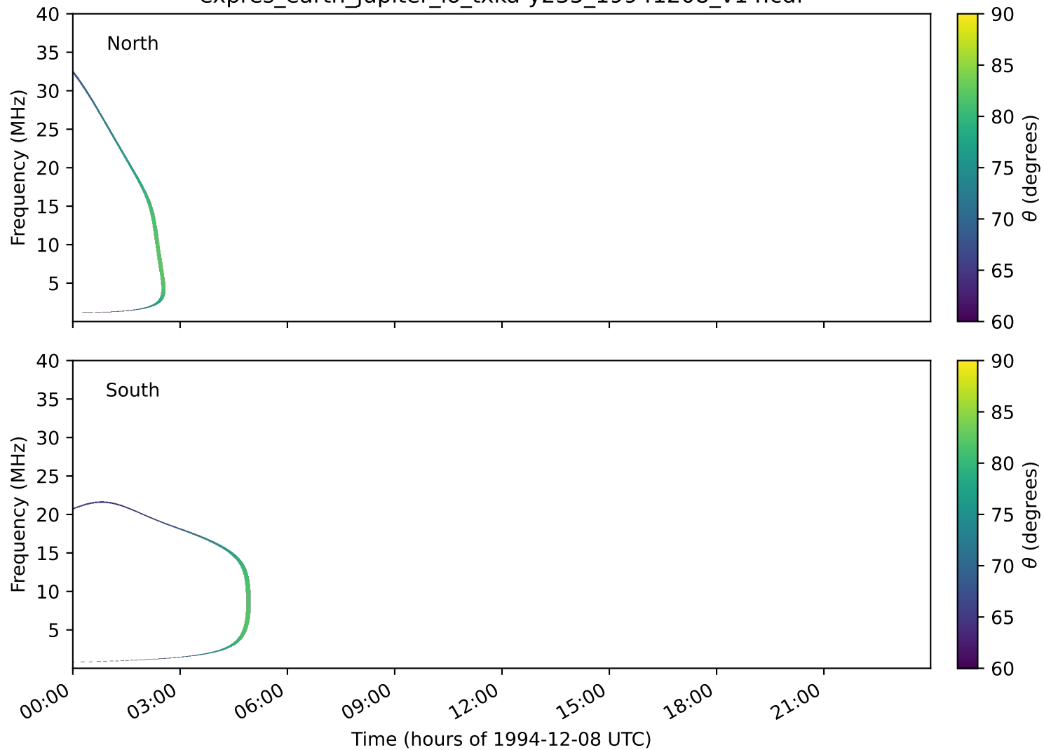
expres_earth_jupiter_io_txka-y235_19941208_v14.cdf
