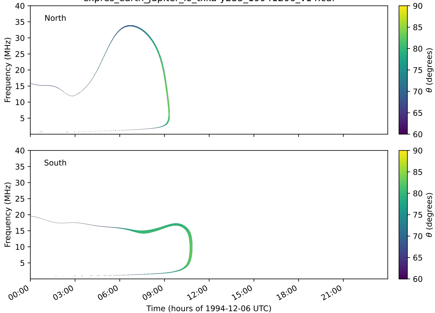
expres_earth_jupiter_io_txka-y235_19941206_v14.cdf
