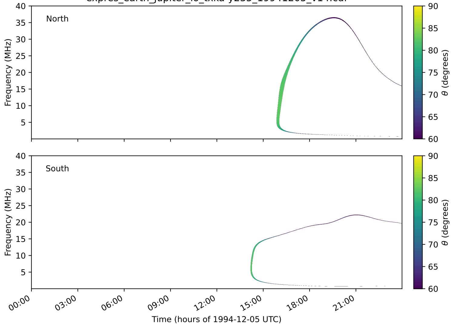
expres_earth_jupiter_io_txka-y235_19941205_v14.cdf
