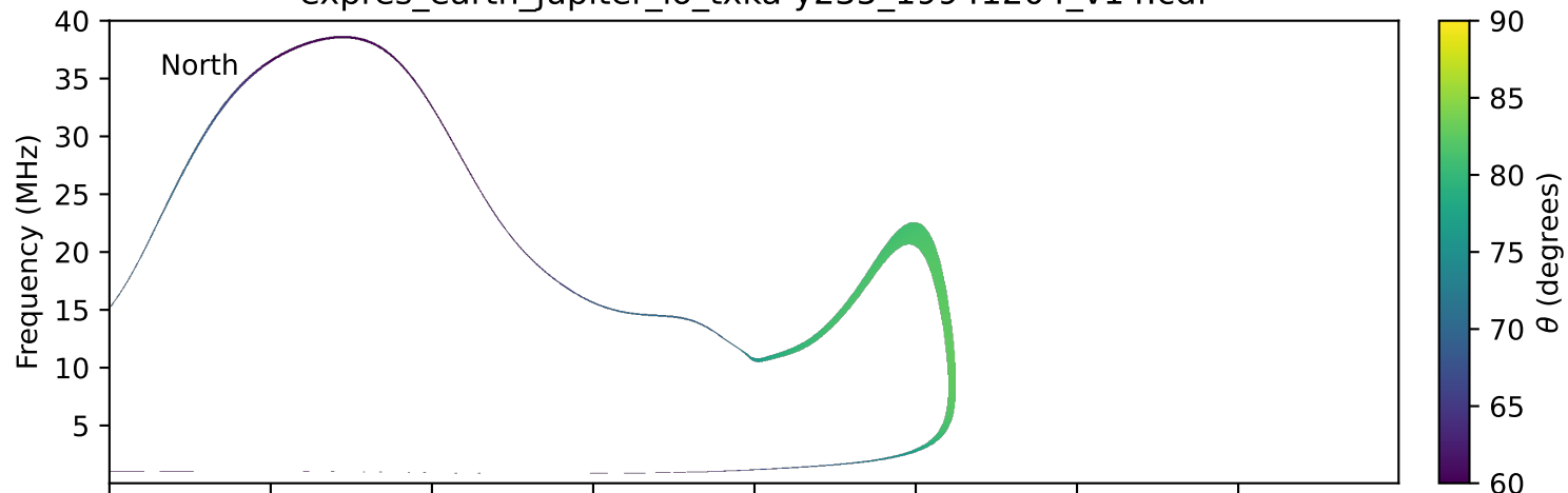
expres_earth_jupiter_io_txka-y235_19941204_v14.cdf
