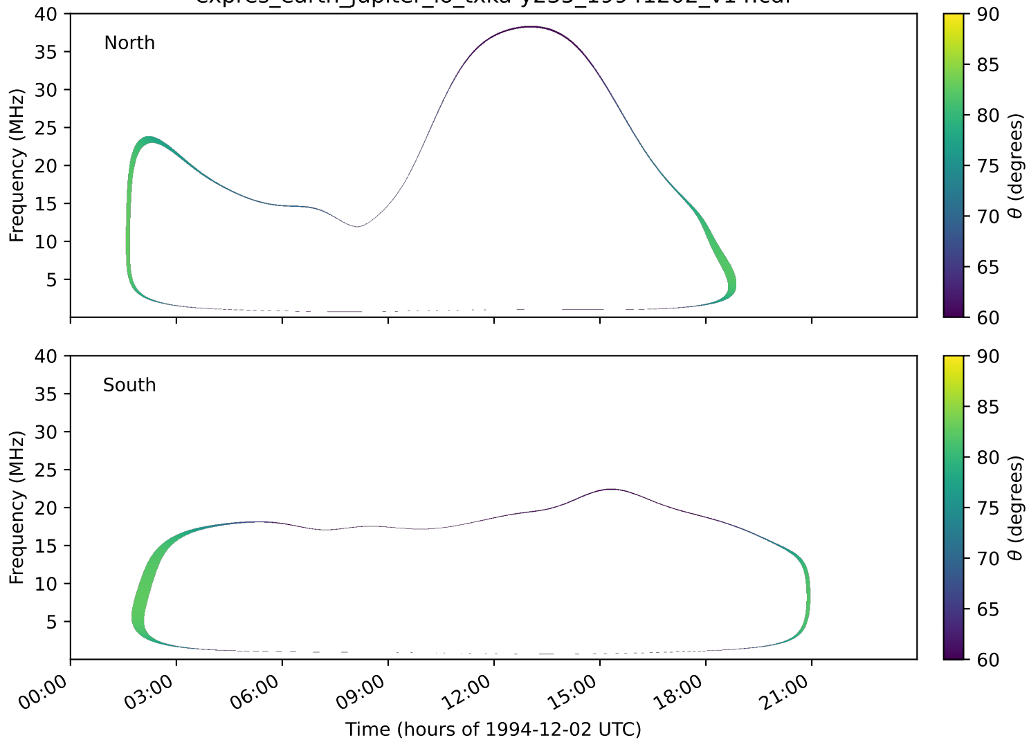
expres_earth_jupiter_io_txka-y235_19941202_v14.cdf
