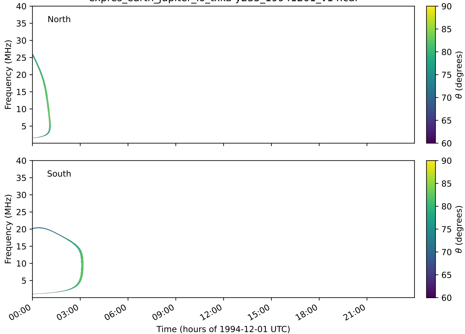
expres_earth_jupiter_io_txka-y235_19941201_v14.cdf
