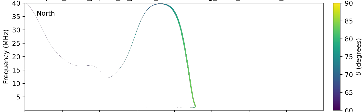
expres_earth_jupiter_io_jrm33_lossc-wid1deg_3kev_19941229_v11.cdf
