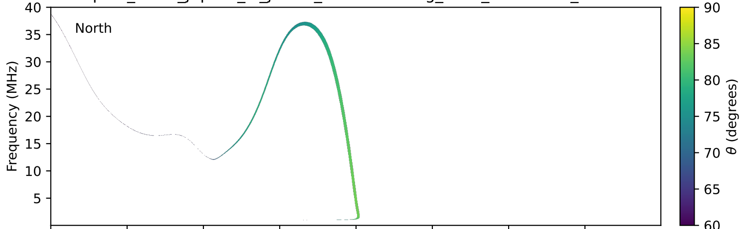
expres_earth_jupiter_io_jrm33_lossc-wid1deg_3kev_19941222_v11.cdf
