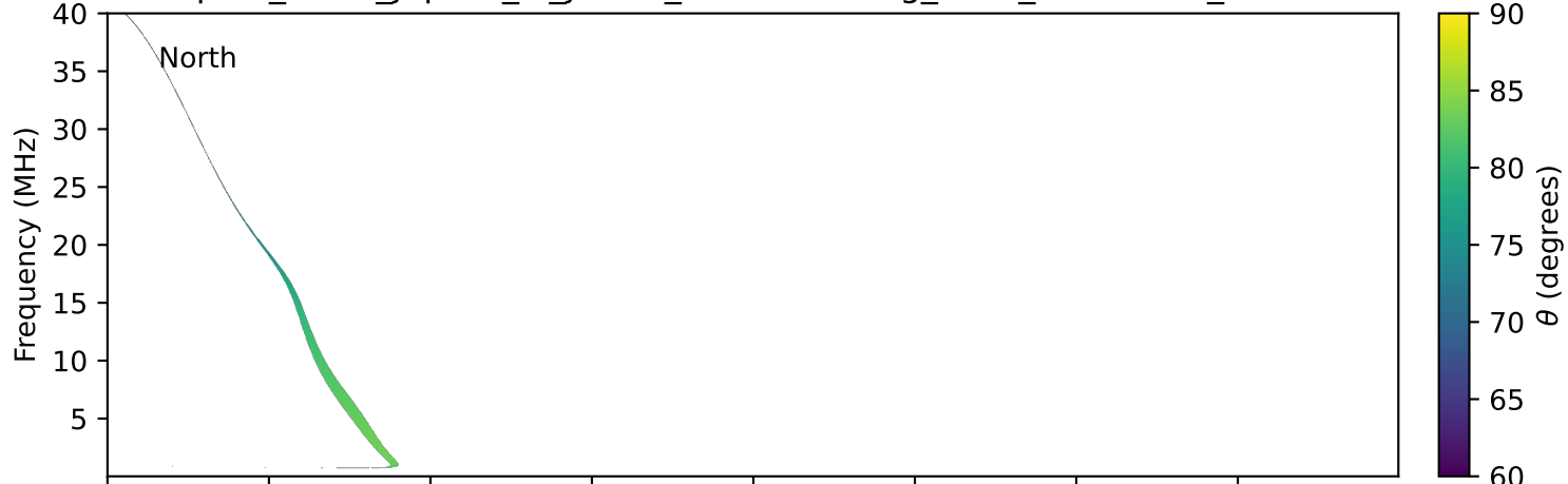
expres_earth_jupiter_io_jrm33_lossc-wid1deg_3kev_19941215_v11.cdf
