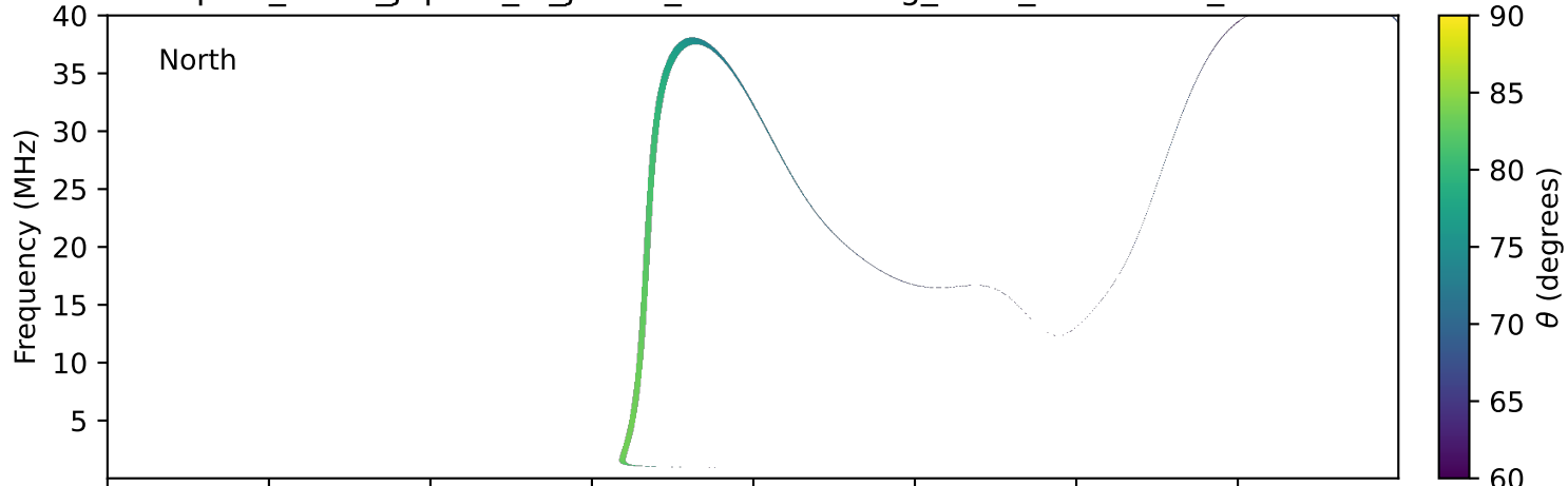
expres_earth_jupiter_io_jrm33_lossc-wid1deg_3kev_19941207_v11.cdf
