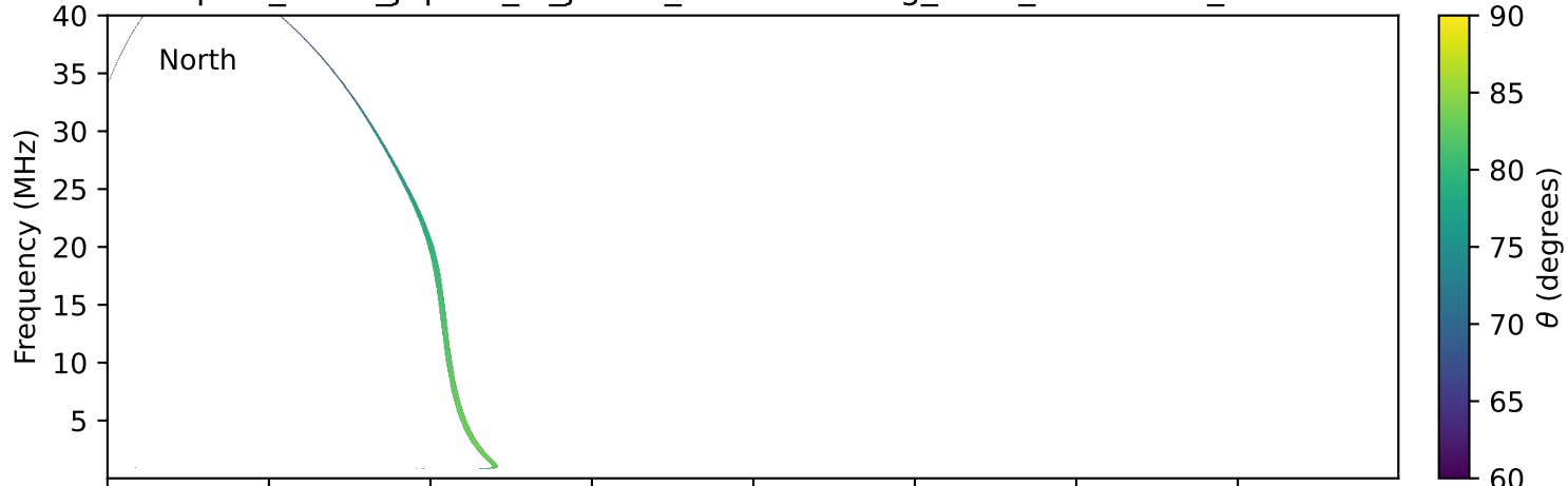
expres_earth_jupiter_io_jrm09_lossc-wid1deg_3kev_19941231_v11.cdf
