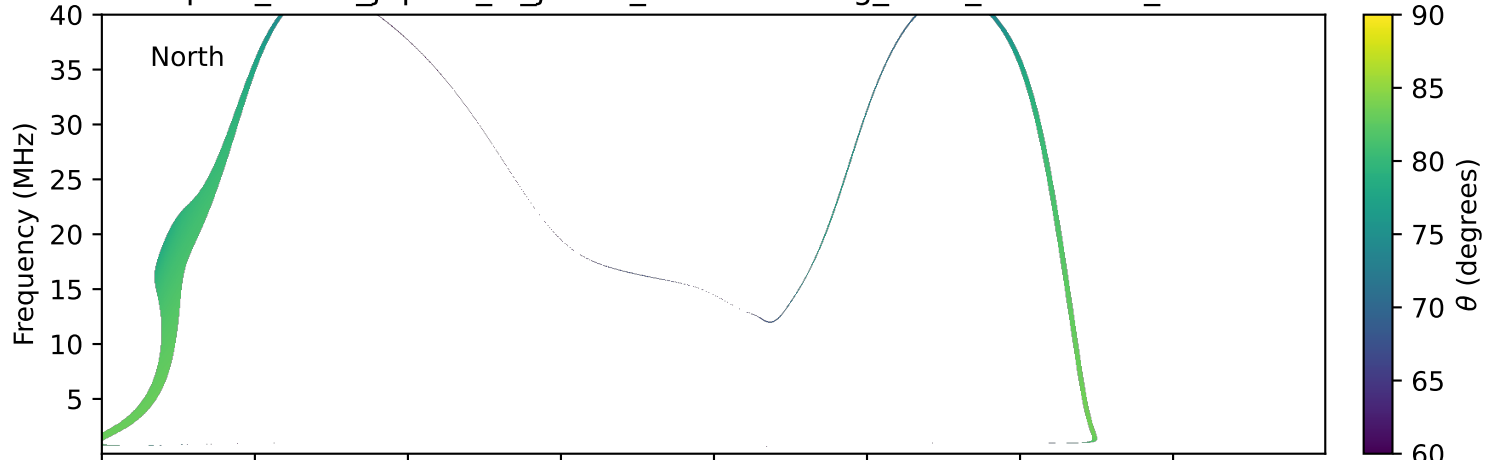
expres_earth_jupiter_io_jrm09_lossc-wid1deg_3kev_19941218_v11.cdf
