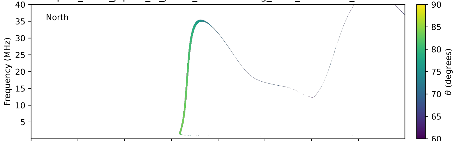
expres_earth_jupiter_io_jrm09_lossc-wid1deg_3kev_19941207_v11.cdf
