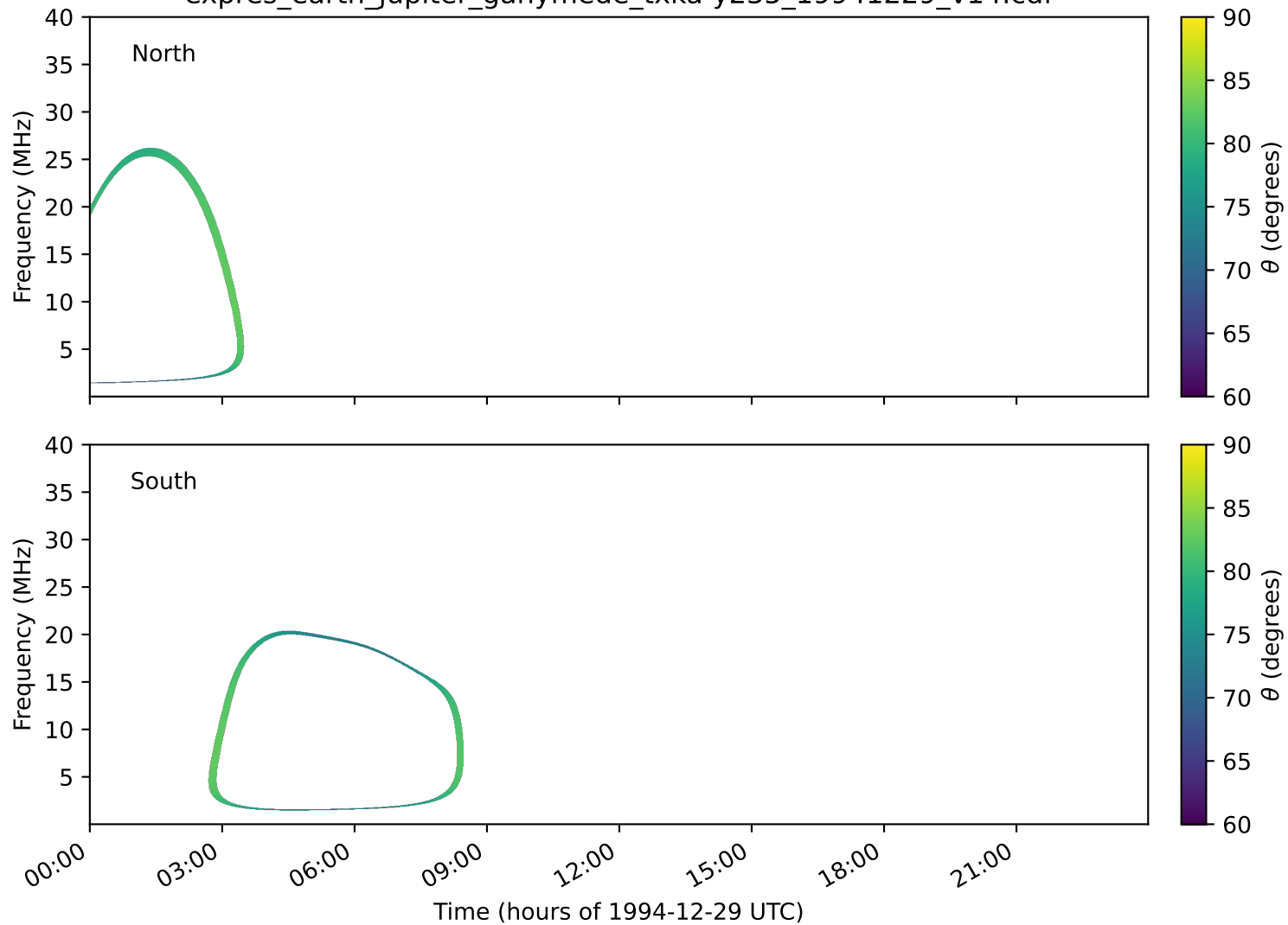
expres_earth_jupiter_ganymede_txka-y235_19941229_v14.cdf
