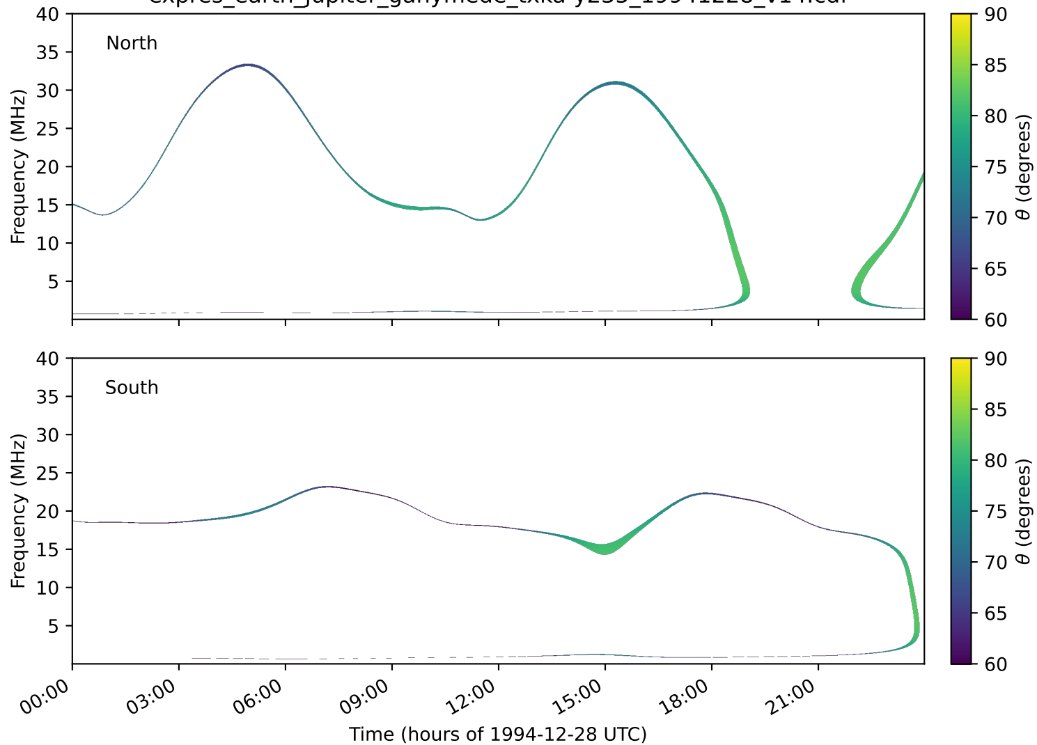
expres_earth_jupiter_ganymede_txka-y235_19941228_v14.cdf
