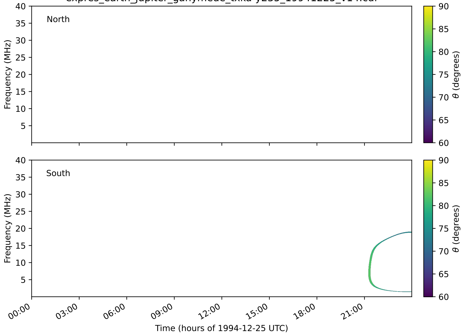
expres_earth_jupiter_ganymede_txka-y235_19941225_v14.cdf
