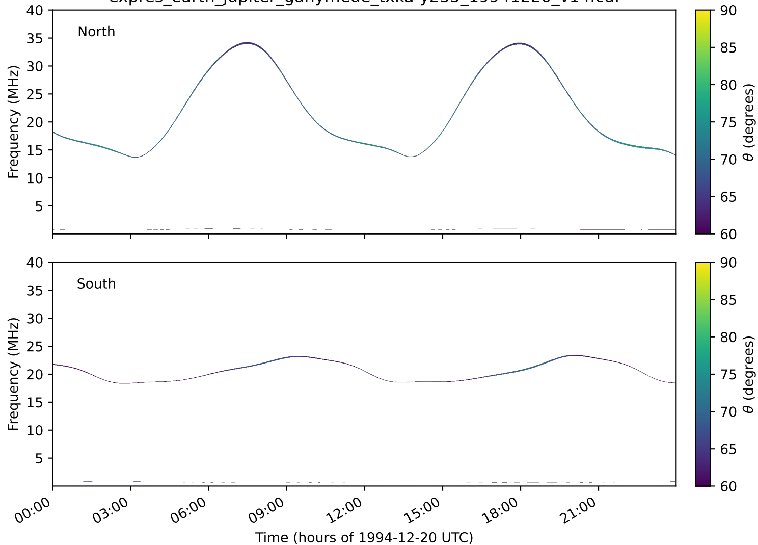
expres_earth_jupiter_ganymede_txka-y235_19941220_v14.cdf
