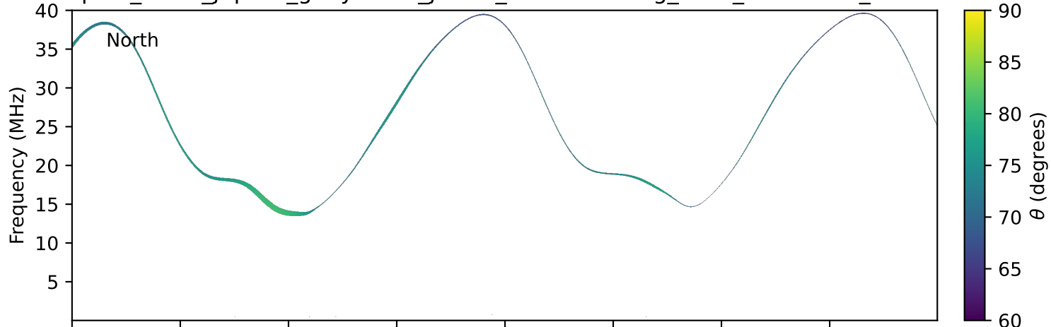
expres_earth_jupiter_ganymede_jrm33_lossc-wid1deg_3kev_19941219_v11.cdf
