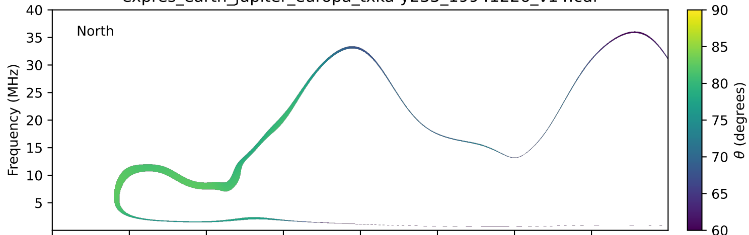
expres_earth_jupiter_europa_txka-y235_19941226_v14.cdf
