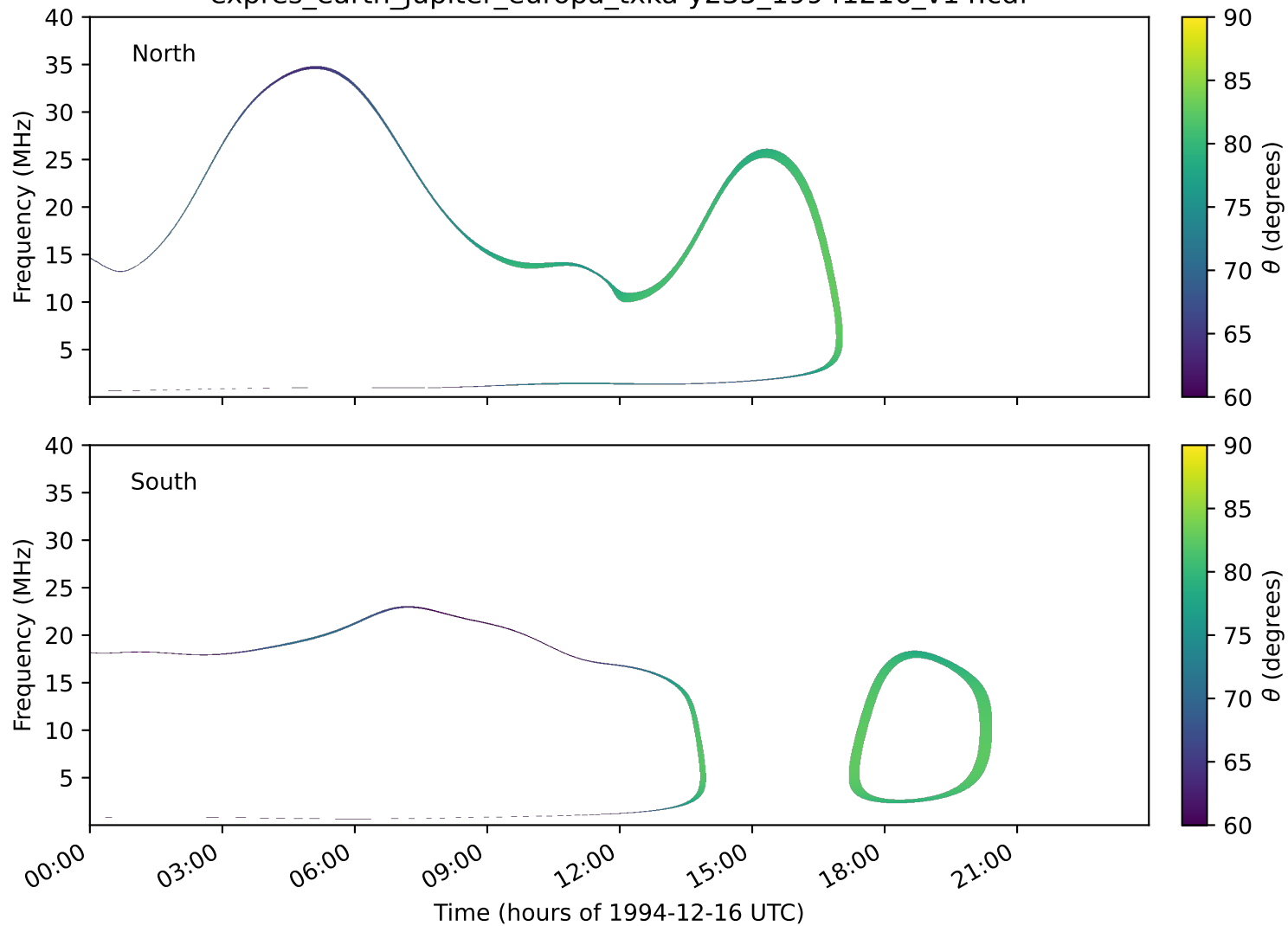
expres_earth_jupiter_europa_txka-y235_19941216_v14.cdf
