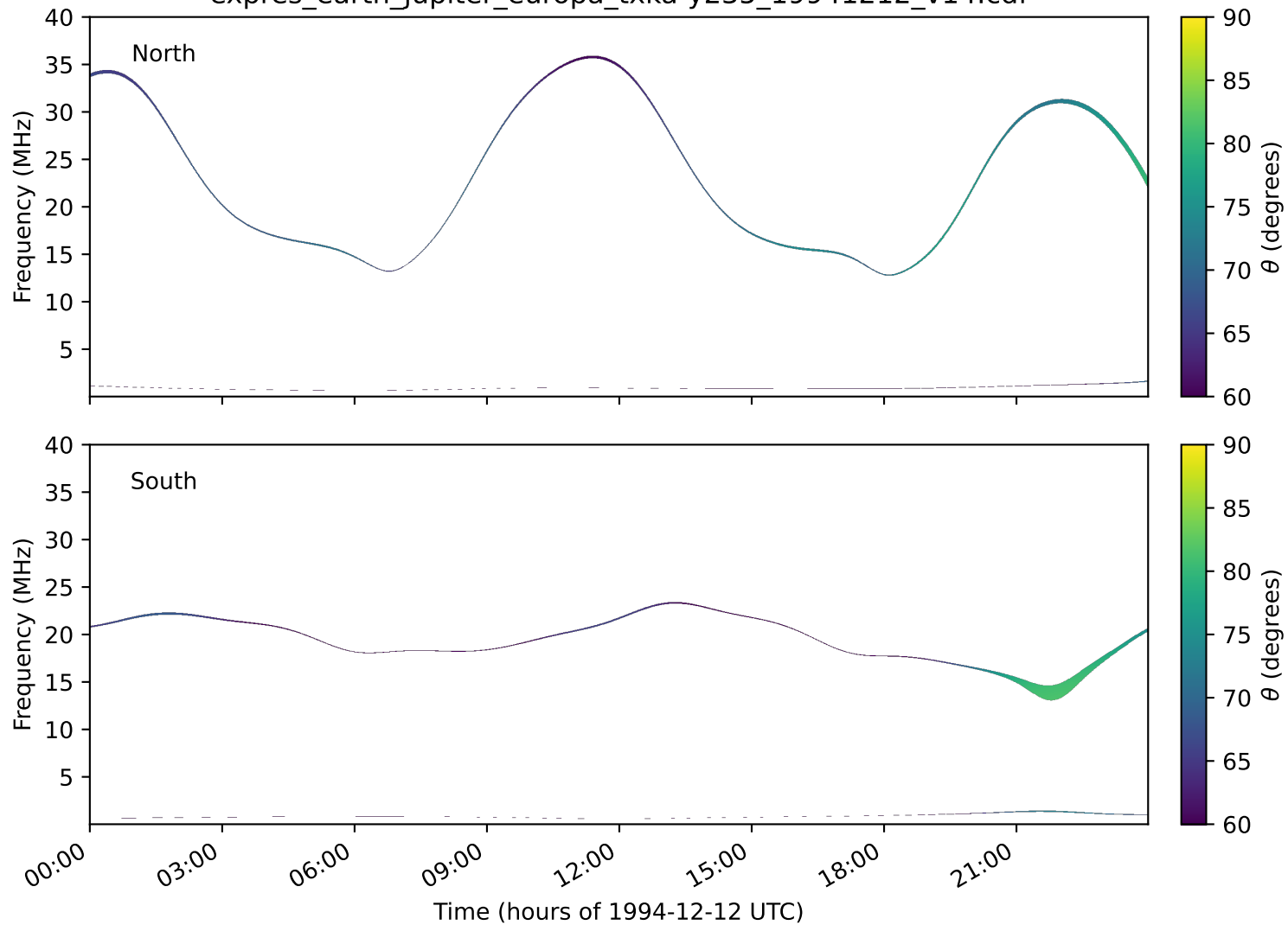
expres_earth_jupiter_europa_txka-y235_19941212_v14.cdf
