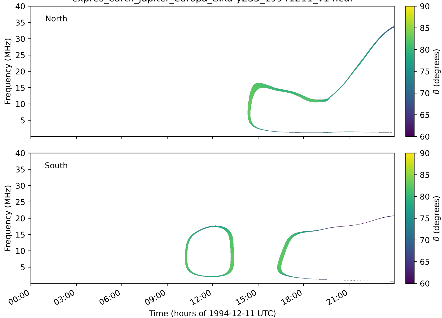
expres_earth_jupiter_europa_txka-y235_19941211_v14.cdf
