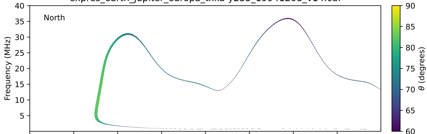
expres_earth_jupiter_europa_txka-y235_19941208_v14.cdf
