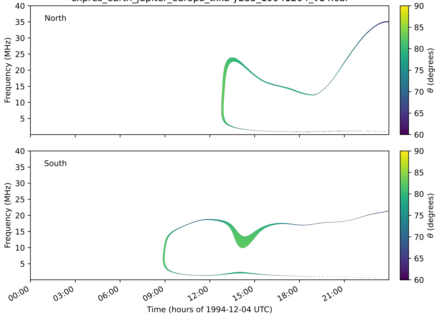
expres_earth_jupiter_europa_txka-y235_19941204_v14.cdf
