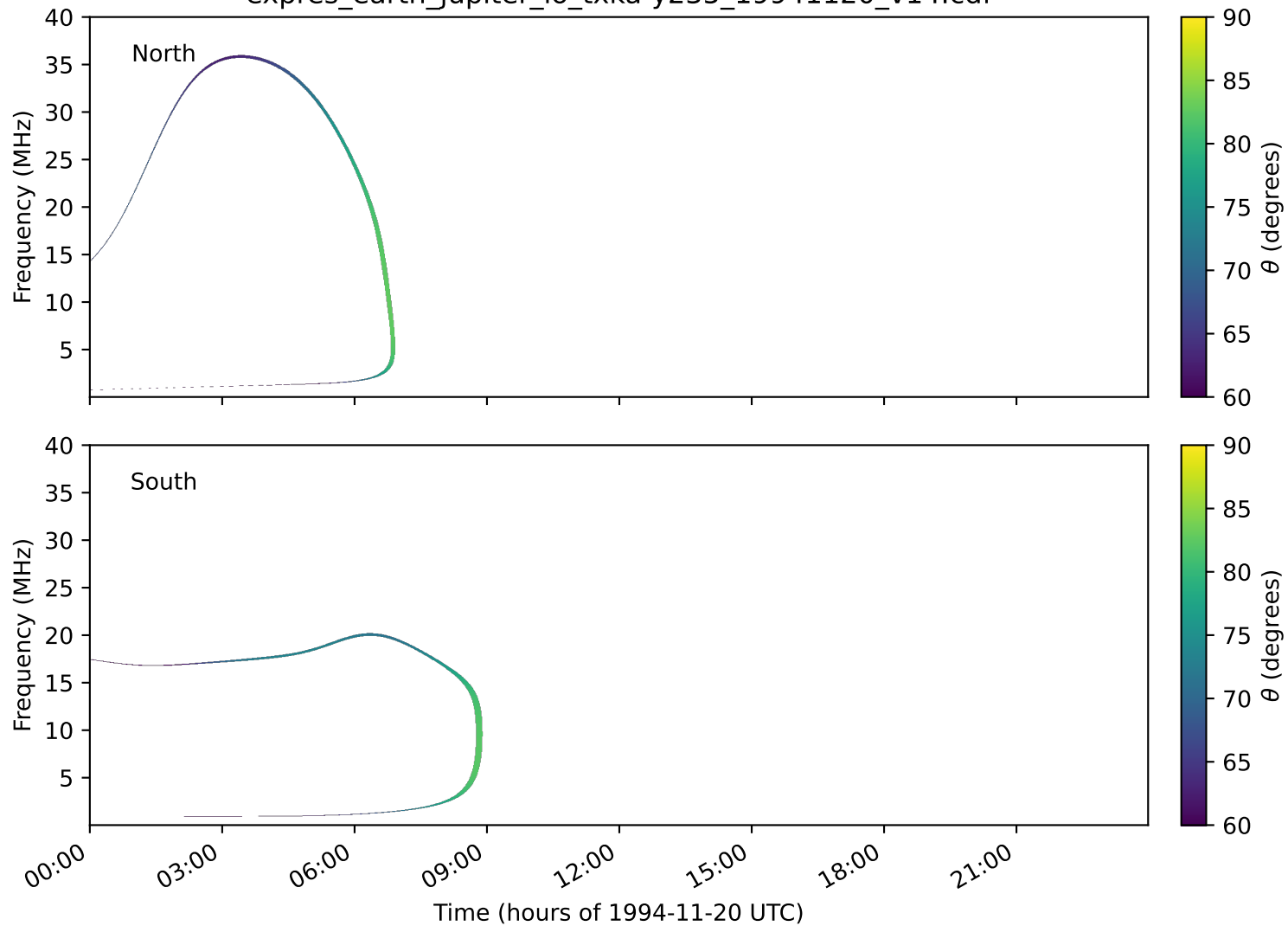
expres_earth_jupiter_io_txka-y235_19941120_v14.cdf
