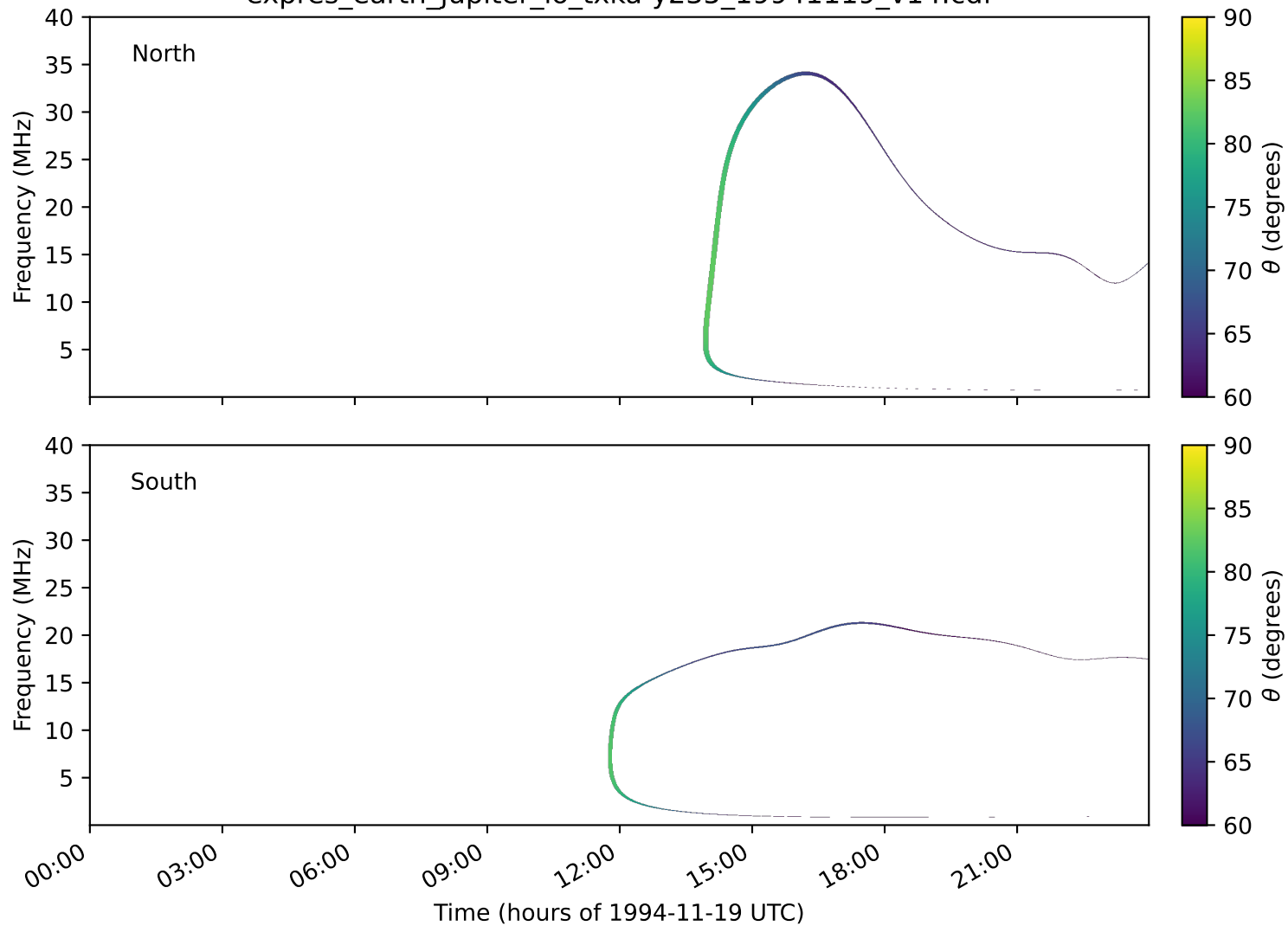
expres_earth_jupiter_io_txka-y235_19941119_v14.cdf
