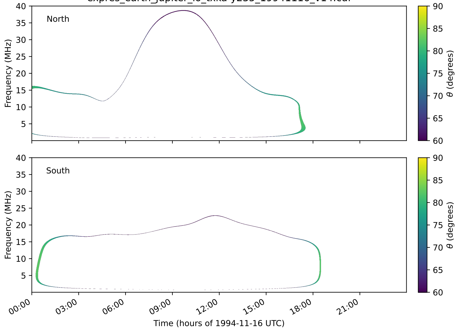
expres_earth_jupiter_io_txka-y235_19941116_v14.cdf
