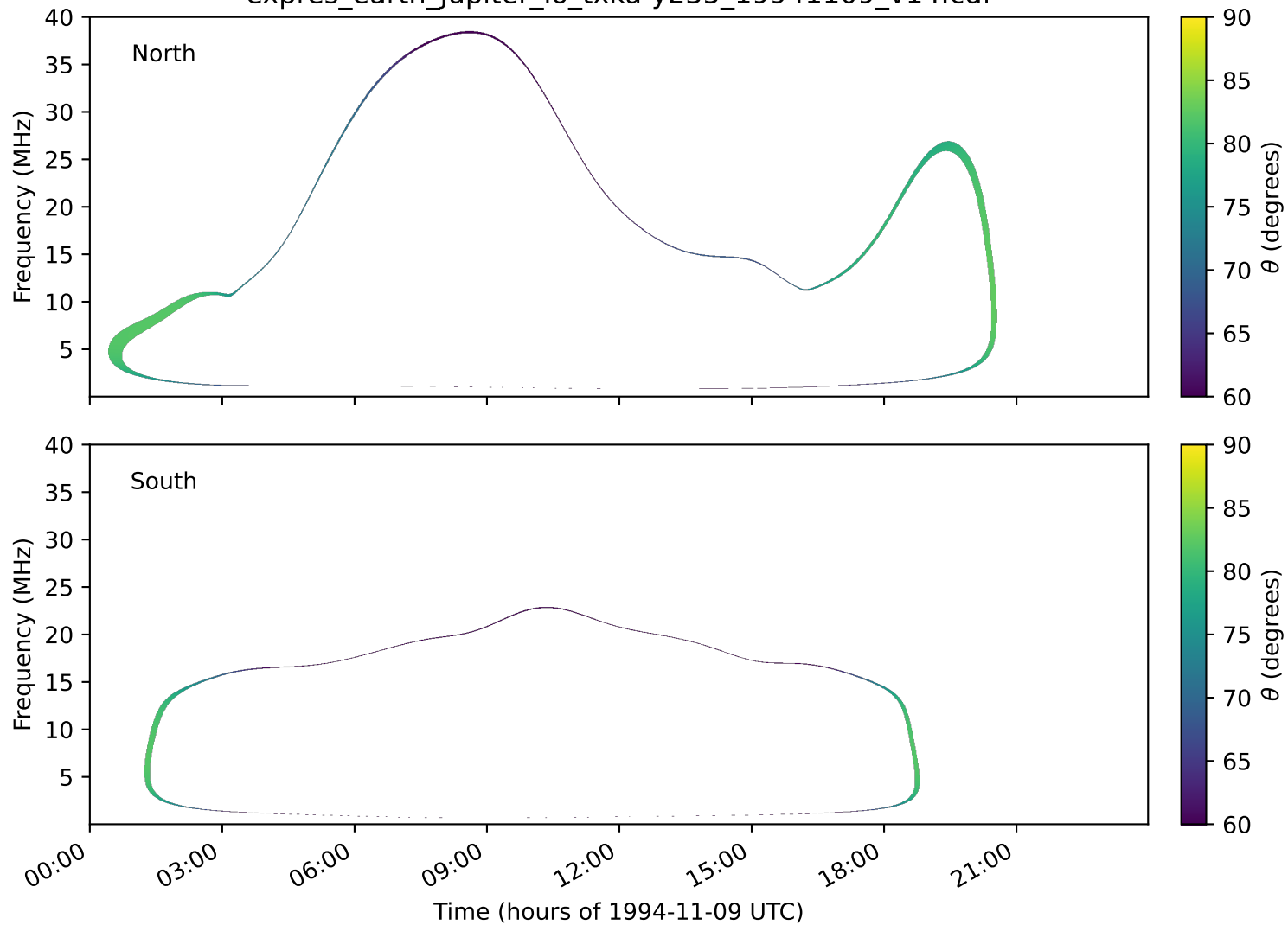
expres_earth_jupiter_io_txka-y235_19941109_v14.cdf
