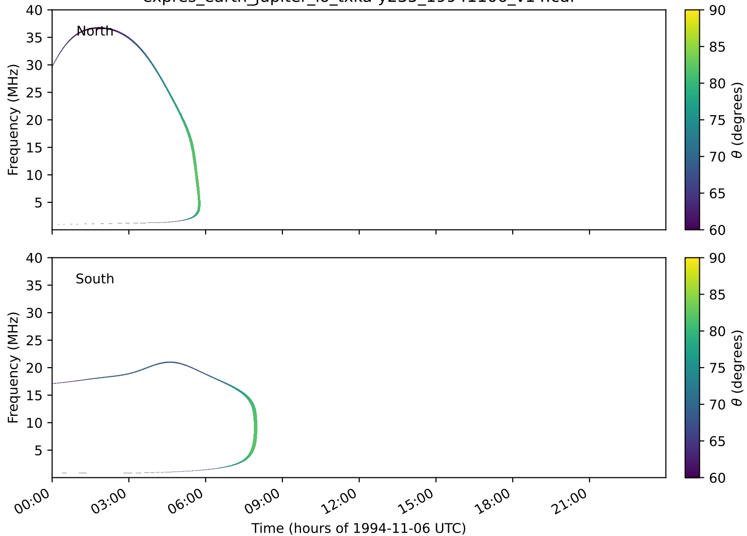
expres_earth_jupiter_io_txka-y235_19941106_v14.cdf
