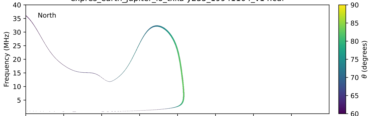
expres_earth_jupiter_io_txka-y235_19941104_v14.cdf
