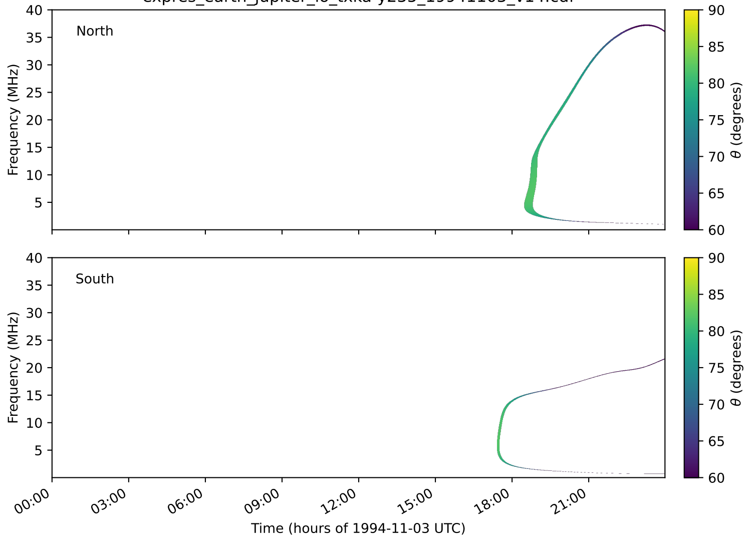
expres_earth_jupiter_io_txka-y235_19941103_v14.cdf
