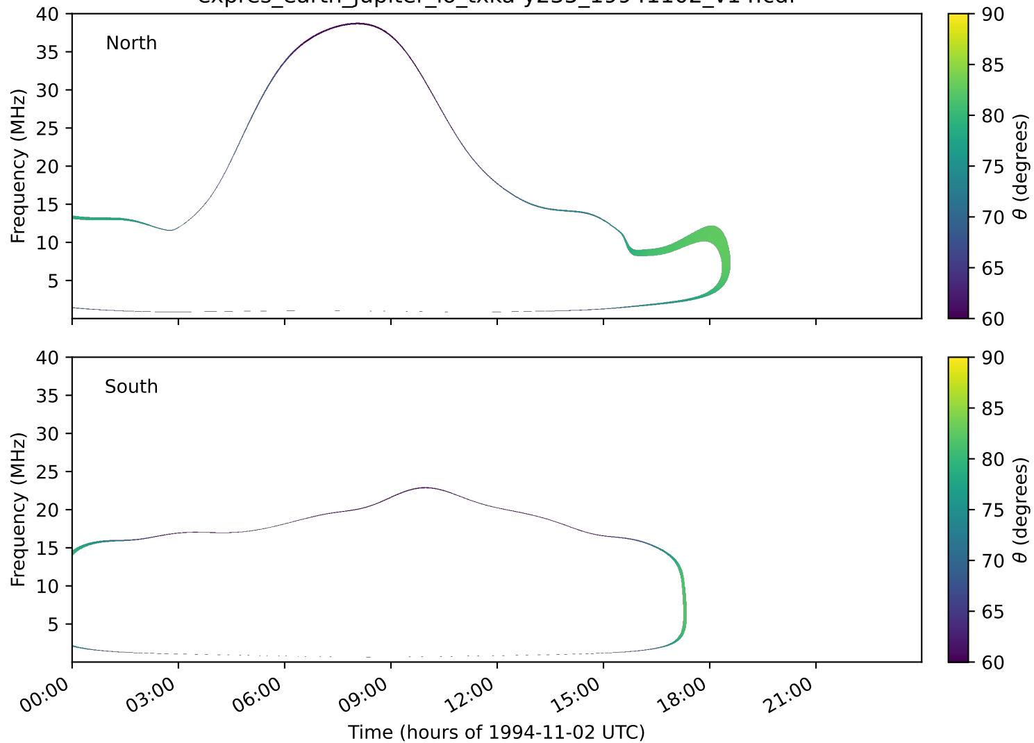
expres_earth_jupiter_io_txka-y235_19941102_v14.cdf
