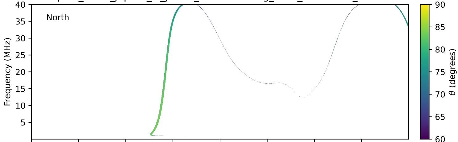
expres_earth_jupiter_io_jrm33_lossc-wid1deg_3kev_19941130_v11.cdf
